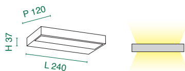
LED Warm white - Natural white 24W - 3225 lm
