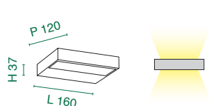
LED Warm white - Natural white 18W - 2570 lm
