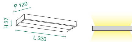
LED Warm white - Natural white 39W - 4990 lm
